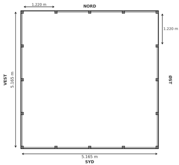
Figur 2. Plantegning.
